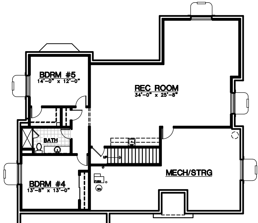
LOWER LEVEL PLAN OPTIONAL FINISHED
